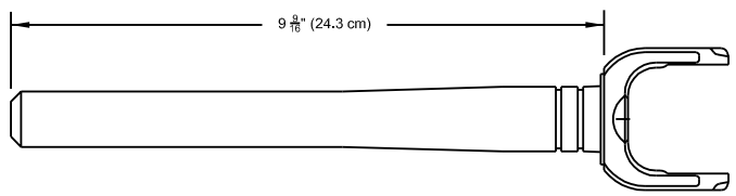
U-Joint Coupling End Yoke (39385A1) used on older in-line models
