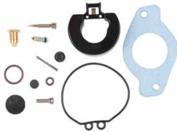
18-7767 KIT CARBURADOR Reemplaza: 6H4-W0093-01-00 (3) de 18-7767 = (1) de 6H4-W0093-01-00
