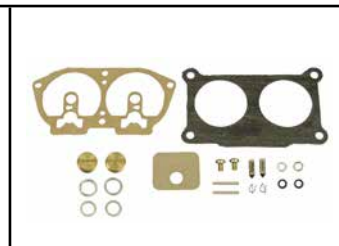
18-7002 KIT CARBURADOR Reemplaza: 6E5-W0093-06-00 Para: 115 (1986-88,1992-93, 1995), 130 (1988,1992-93, 1995), 150, 175 (1986- 87, 1992-95), 200 (1986-87,1992-95), 225 (1992-93)
