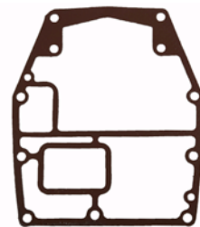
18-99151 JUNTA CÁRTER SUPERIOR Reemplaza: 688-45113-A0 Para: 90(1984-09), B90(1997-99), C75(1994-99), C80(1997), C85(1991-96), C90(1997-01), C85(1989-90), E75(1995-00), P75(1996-99)
