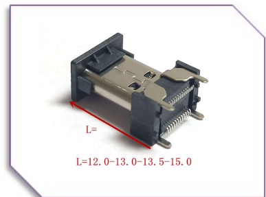
A25-F-M-C-24 USB Type C 24pin Female SMT Type
