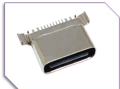
A25WP-F-M-A-12 Waterproof USB Type C 12pin Female SMT Type
