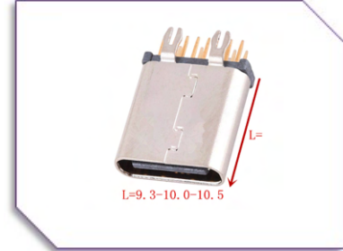
A25-F-V-B-14 USB Type C 14pin Female Vertical Dip Type
