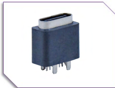
A25WP-F-D-A-14 Waterproof USB Type C 14pin Female Dip Type
