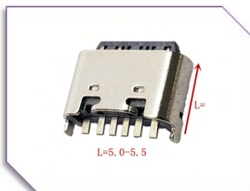
A25-F-V-A-6 USB Type C 6pin Female Vertical Dip Type
