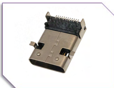
A25-F-DM-C-24 USB Type C 24pin Female Dip & SMT Type
