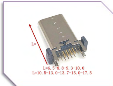
A25-F-V-A-16 USB Type C 16pin Female Vertical Dip Type
