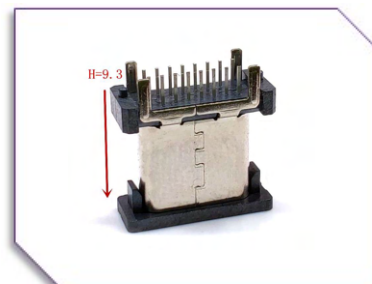
A25-F-V-D-16 USB Type C 16pin Female Vertical Dip Type
