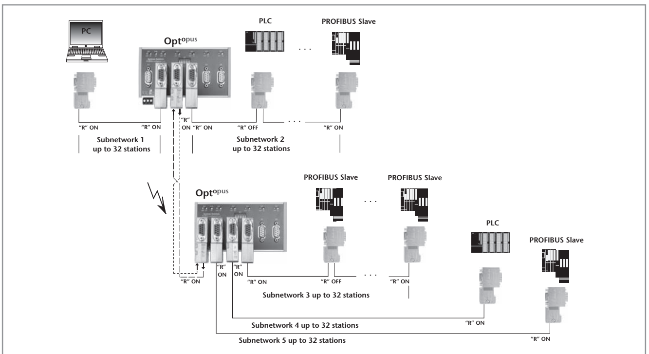
Establishment of a link between two repeaters that is not subject to EMC interference.
