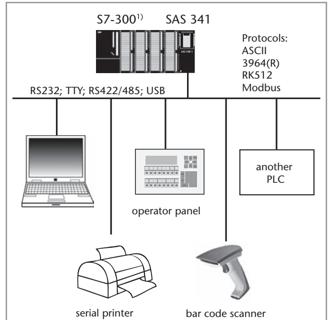
Application example for SAS 341
