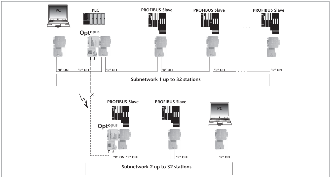
Generation of a completely electrically isolated subnetwork.
