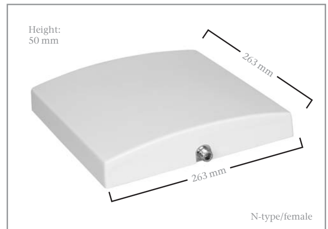
Panel 18 dBi antenna
