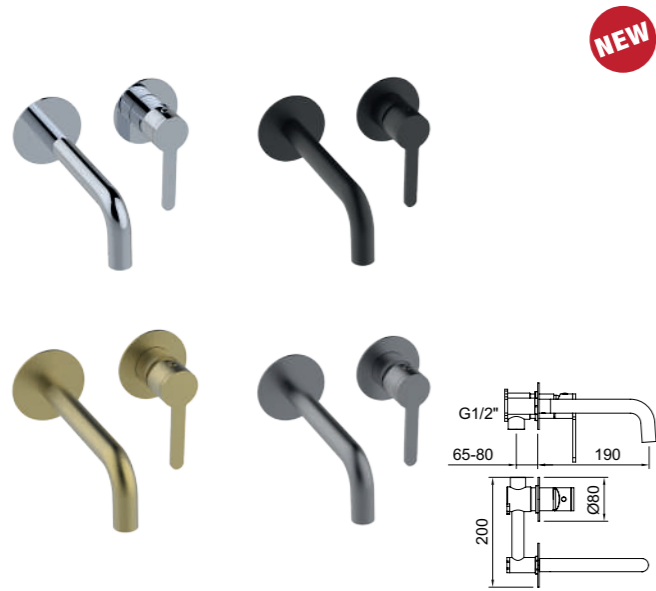
Lavabo empotrar 1/2" con aireador. Concealed basin mixer 1/2" with aerator.
