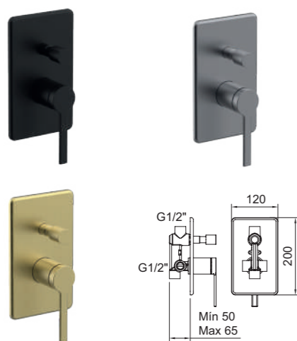
Ducha monomando empotrar 1/2". Concealed single-lever shower mixer 1/2".
