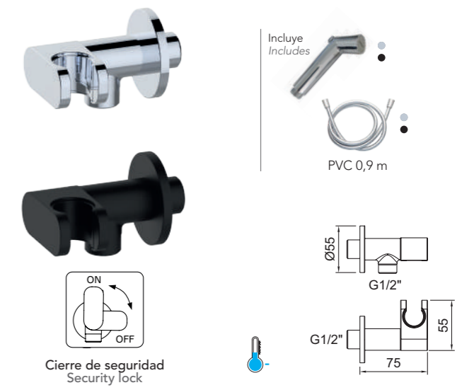
Ducha higiénica mural con soporte integrado. Wall mounted shattaf with support included.
