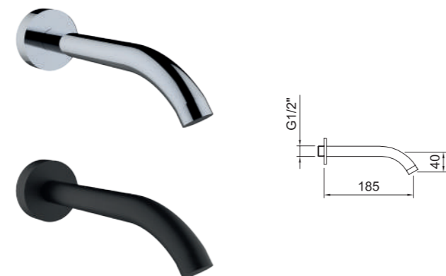
Caño mural Caiman. 185mm Bath spout Caiman. 185mm
