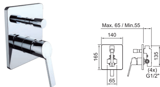
Ducha monomando empotrar 1/2". Concealed single-lever shower mixer 1/2".
