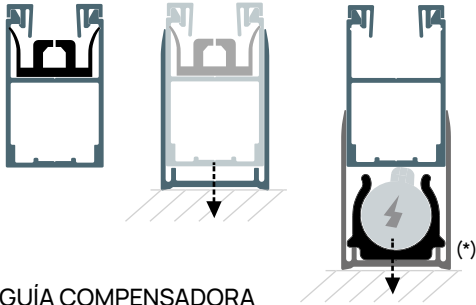
GUÍA COMPENSADORA COULISSE COMPENSATOIRE Counter-balancing fitting for the guide rail
