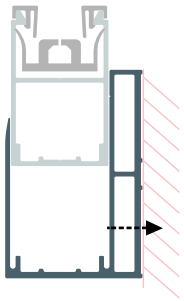
GUÍA COMPENSADORA DE PARED COULISSE COMPENSATOIRE MURALE Wall counter-balancing fitting for the guide rail
