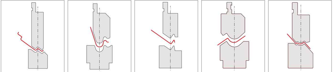
GROUP - A / STAMPI SPECIALI MONOLITICI - DIMENSIONI MASSIME: PUNZONE 140mm x 60mm - MATRICE 120mm x 100mm MONOLITHIC SPECIAL TOOLS - MAX. DIMENSIONS: PUNCH 140mm x 60mm / DIE 120mm x 100mm
